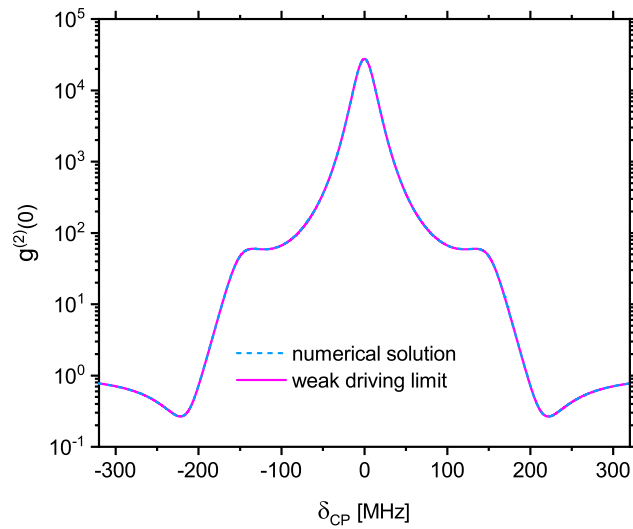
Figure 1: This figure illustrates the second-order coherence function curves for specified values versus probe laser detuning from the atomic resonance. The dashed curve corresponds to equation (2.16), while the solid curve corresponds to equation (3.18).
